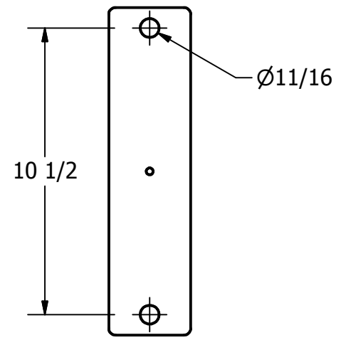
VIEW C-C FOOT PAD
